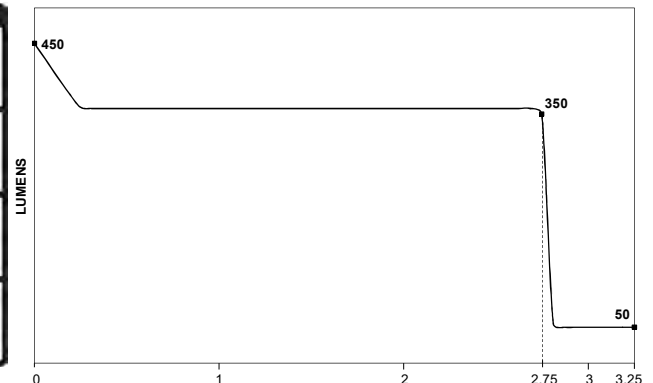
SL-20L / SL-20LP PERFORMANCE CURVE
